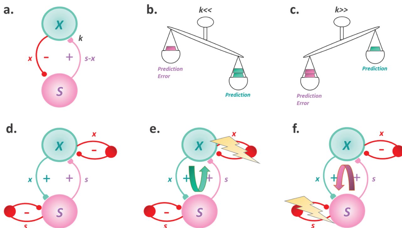
Fig. 1. Illustration of different Bayesian models of hallucinations. (a–c) The predictive coding framework. (d–f) The circular inference framework. X , hidden cause; S , sensory variable; x and s , predictions and sensory messages; s-x , prediction error; k , relative weight of inputs as compared to predictions (Kalman gain).
